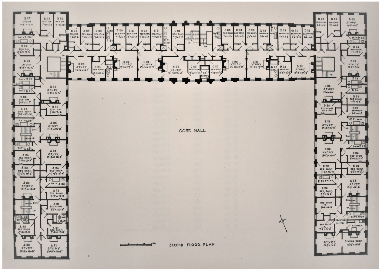
Figure B.IX Floor Plan
